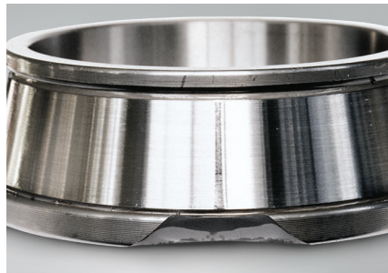
Part: Inner ring of a tapered roller bearing Observation: Fracture occurs at the cone back face rib surface Cause: Large shock during mounting
