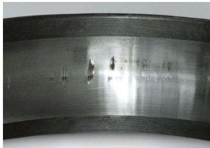
Part: Outer ring of Photo 6.12.1
